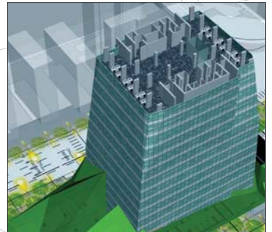
horizontal section
